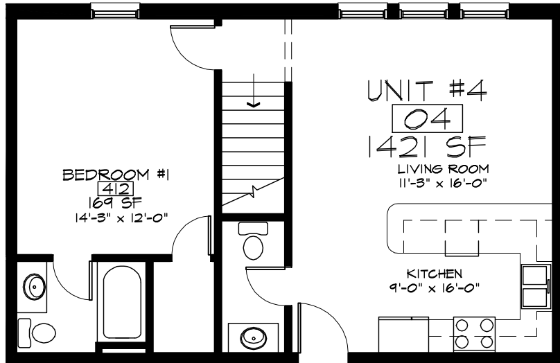
2 SECOND LEVEL NOT TO SCALE
