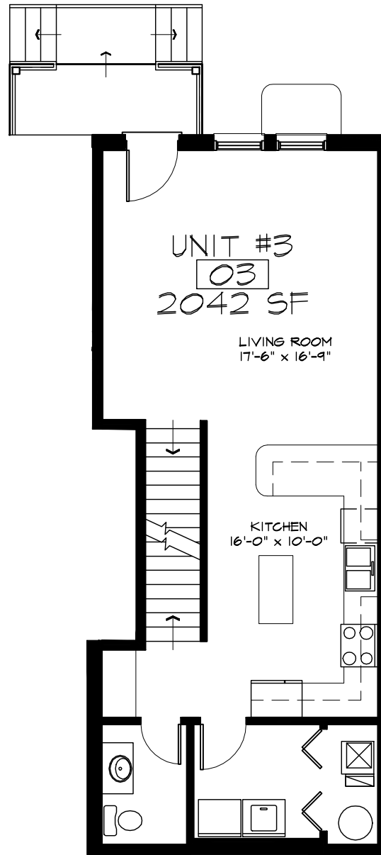
1 FIRST LEVEL NOT TO SCALE
