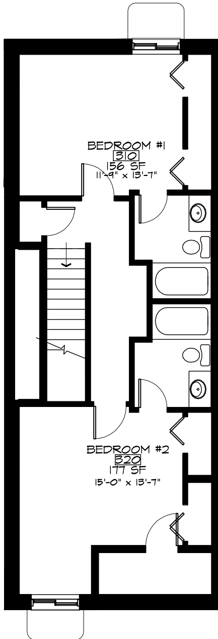
0 LOWER LEVEL NOT TO SCALE
