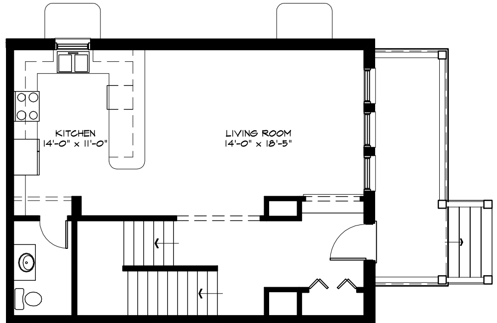
1 FIRST LEVEL NOT TO SCALE
